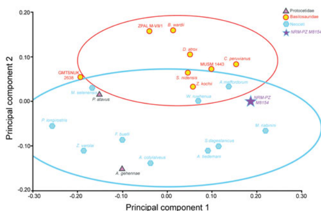
Fig. 5. Variation in vertebral centrum shape among cetaceans compared with NRM-PZ M8154, principal component 1 vs principal component 2; 90% confidence intervals for Basilosauridae and Neoceti are shown with ellipses.
