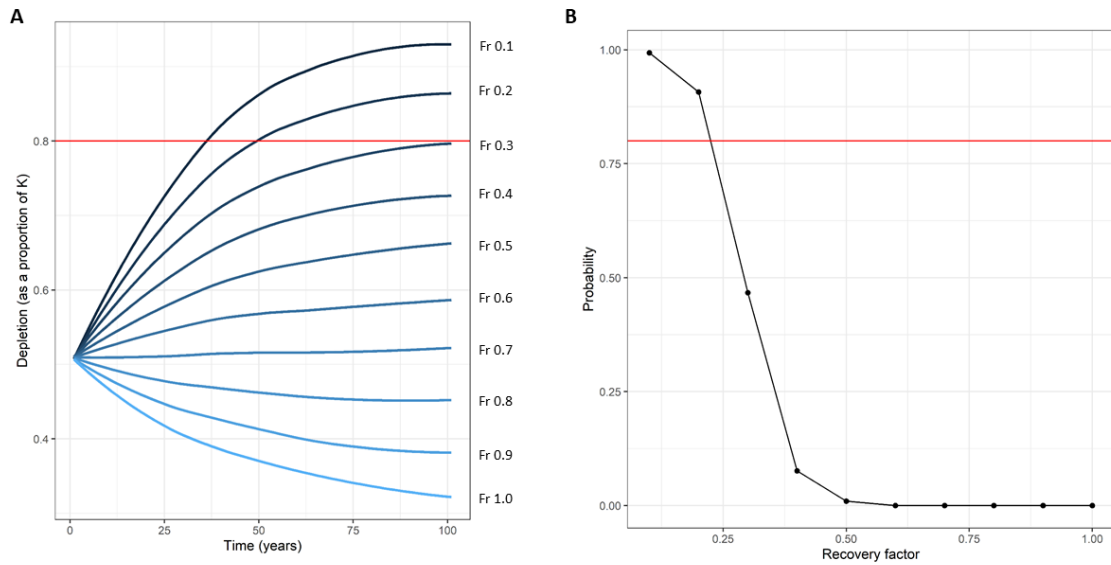
Figure 1: Mean trajectories of depletion level for the Belt Sea population of harbour porpoises ( Phocoena phocoena ) over 100 years of management with various levels of recovery factors ( F_r ) (A). The probability that the population will achieve the conservation objective of reaching 80% of carrying capacity (red line panel A) within 100 years is shown (B). Values are shown for the base case scenario that assumes a Maximum Net Productivity Level (MNPL) of 0.5, a population growth rate ( R_{max} ) of 4%, coefficient of variation of the abundance estimate of 0.2, and no bias in any of the factors that could influence the calculation of potential biological removal. Each F_r tested is shown, and only F_r values of 0.1 and 0.2 allow the population to have a >80% probability (red line panel B) of reaching the conservation objective (80% of K within 100 years).
