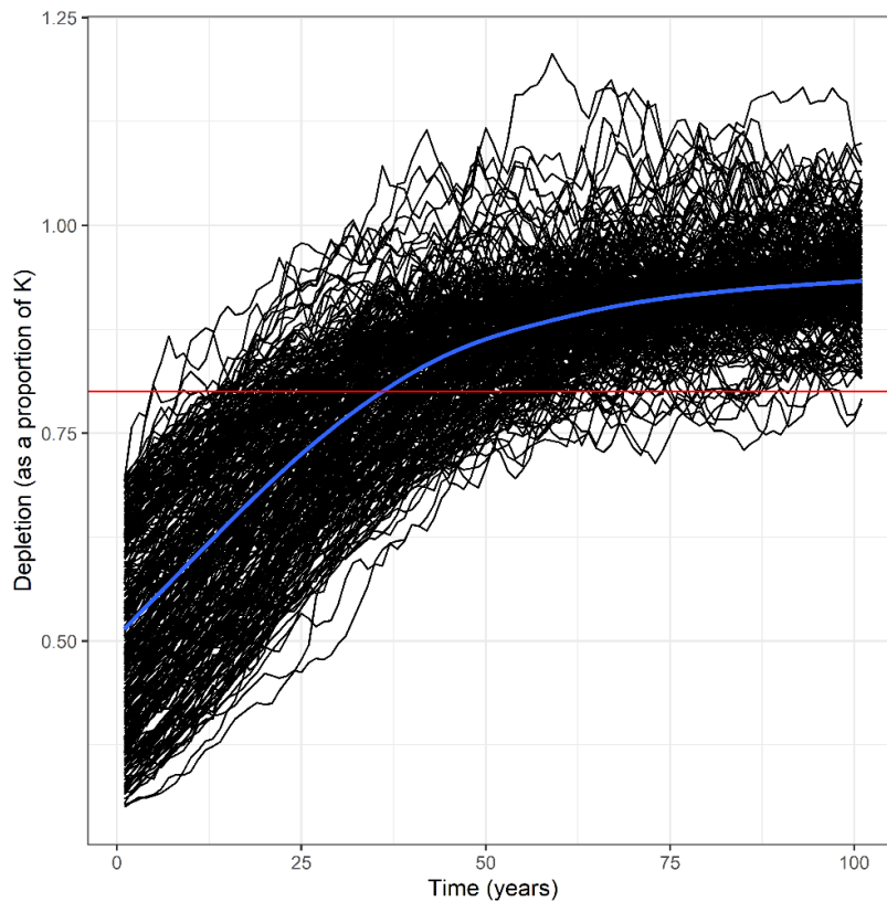
Figure 2: Trajectories of all 302 simulations of the population dynamics of the Belt Sea population under the base case scenario (0A) (assumes a Maximum Net Productivity Level (MNPL) of 0.5, a population growth rate ( R_{max} ) of 4%, coefficient of variation of the abundance estimate of 0.2, and no bias in any of the factors that could influence the calculation of potential biological removal) with a recovery factor of 0.1. The blue line represents the same mean line presented in Figure 1. The red line shows the 80% depletion level of carrying capacity (K), which is in line with the conservation objective of ASCOBANS.
